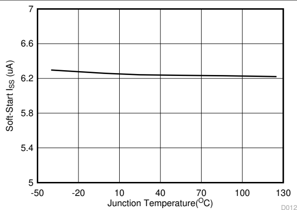
图 5-15. Soft-Start Charge Current Iss vs Junction Temperature
